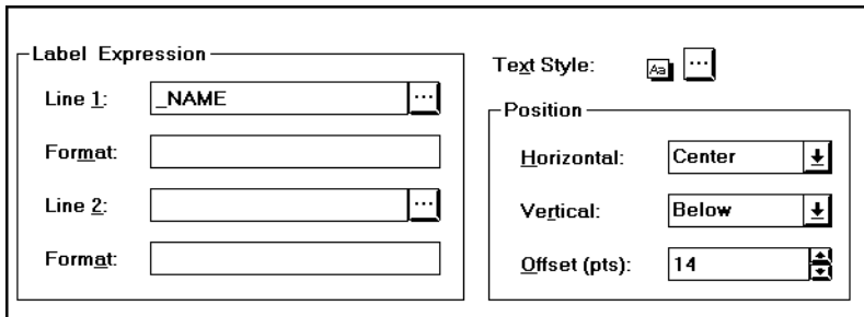
Figure 12.3 Labels subpanel
