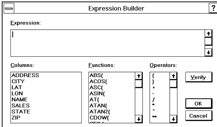
Figure 9.8 Expression Builder
