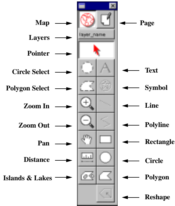
Figure 2.5 Toolbox
