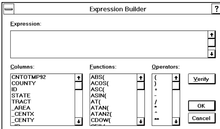
Figure 11.3 Expression Builder
