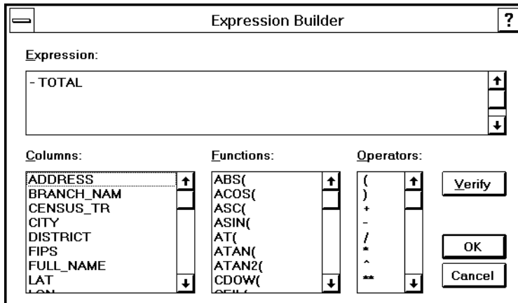
Figure 10.1 Expression Builder
