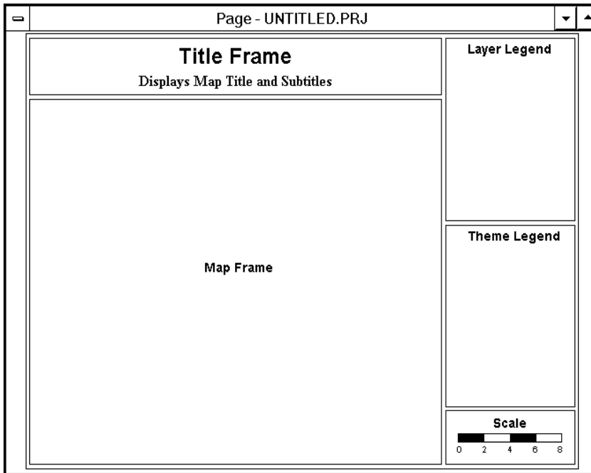
Figure 2.3 Page window
