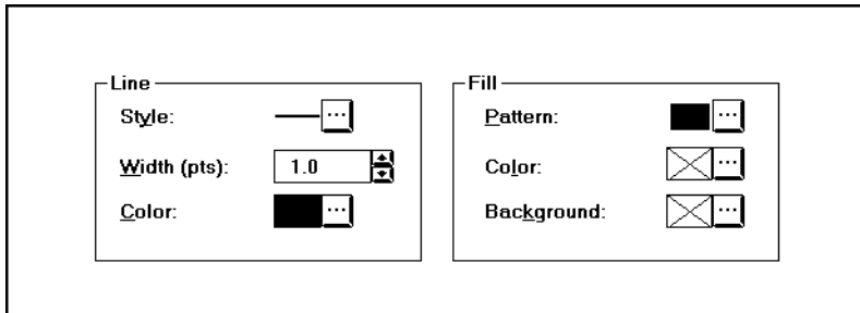
Figure 4.4 Style subpanel
